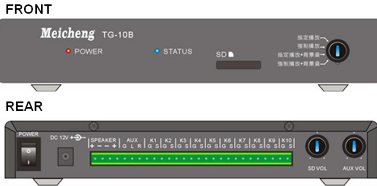
▲ 10 terminals for integrating with any kind of Keypad or Infrared (IR) Sensor
